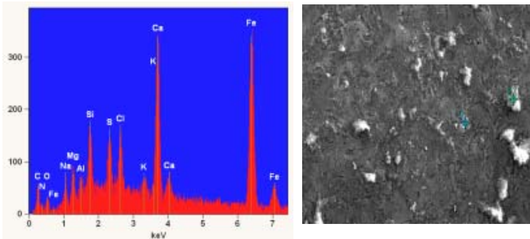
Figure 14 – SEM/EDX analysis of rebar surface of MCI 2020 low density concrete sample after 500 days.
