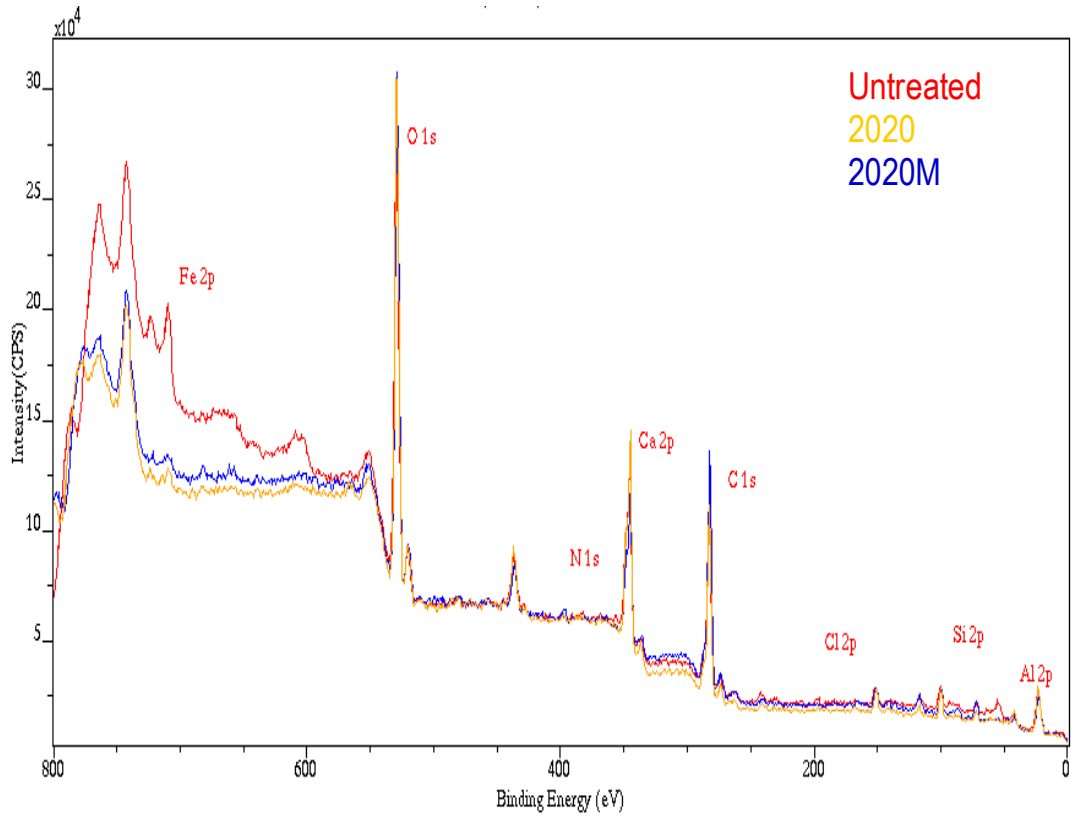
Figure 16 – XPS analysis on concrete samples after 500 days, before etching.
