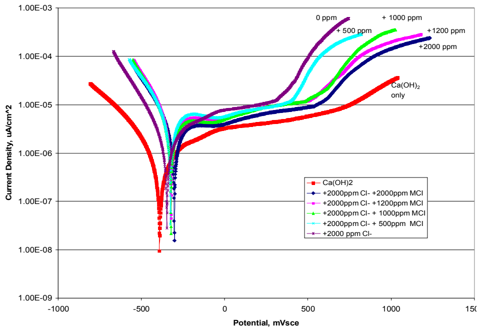
Figure 3 - Polarization behavior of steel rebar in a saturated \text{Ca(OH)}_2 solution with 2000 ppm NaCl and various ppm MCI 2020M additions, pH 12.4, 23 °C.
