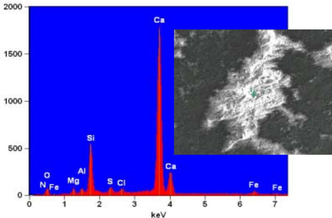
Figure 13 – SEM/EDX analysis of rebar surface of untreated sample after 500 days.
