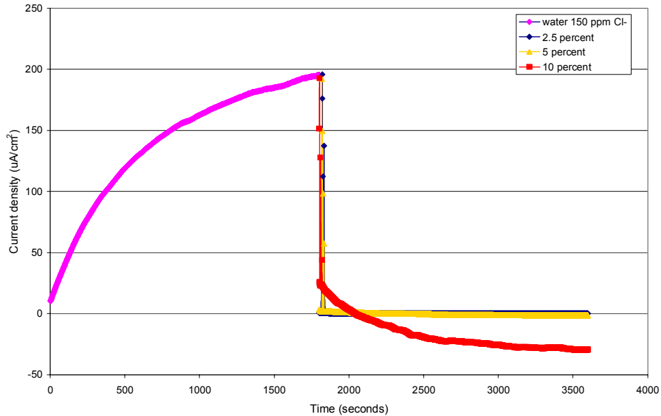
Figure 9 – Potentiostatic Corrosion Behavior of Steel Rebar in Water with Various Concentrations of Migrating Corrosion Inhibitor.
