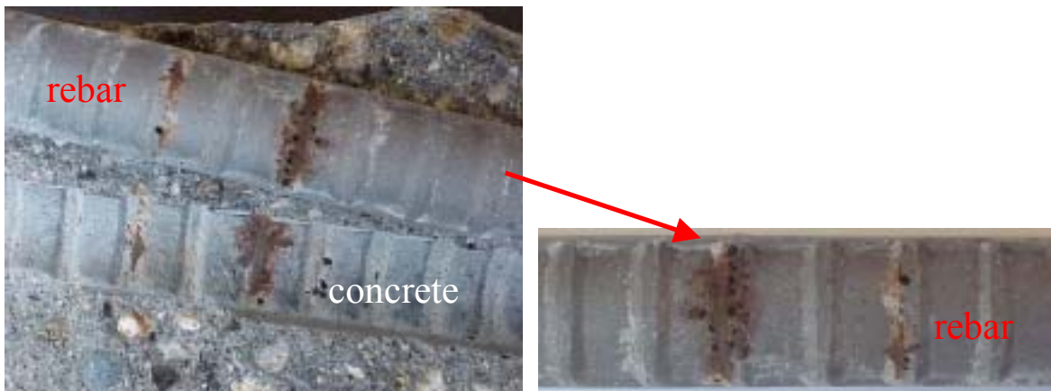
Figure 10 – Untreated low density concrete sample with corrosion rust products near the ribbing of the rebar and stains on the concrete. Photo on the right is an enlargement of the rebar.
