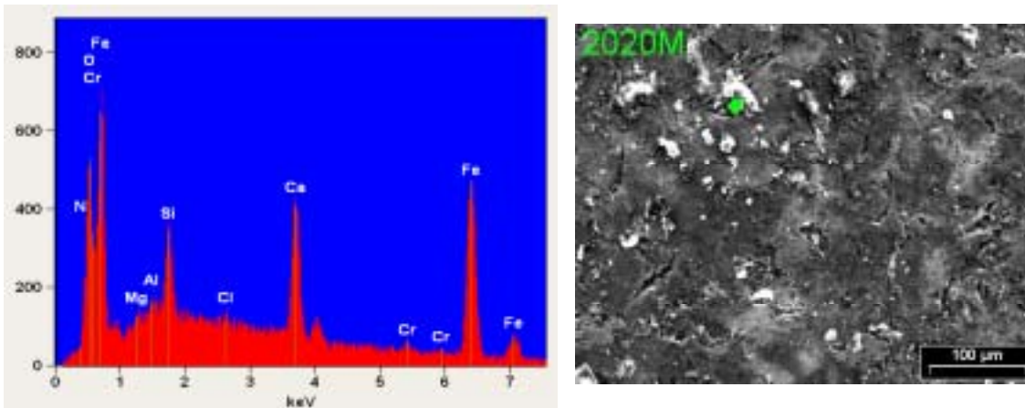
Figure 15 – SEM/EDX analysis of rebar surface of MCI 2020M low density concrete sample after 500 days.
