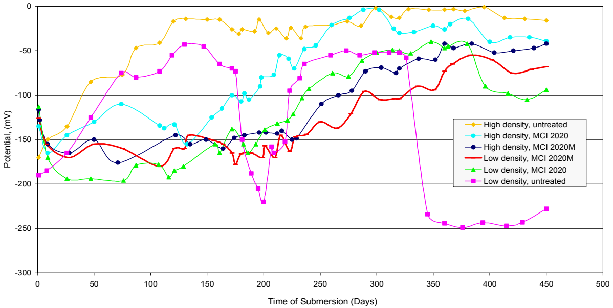
Figure 5 - Comparison of corrosion potential vs time for MCI treated and untreated samples.
