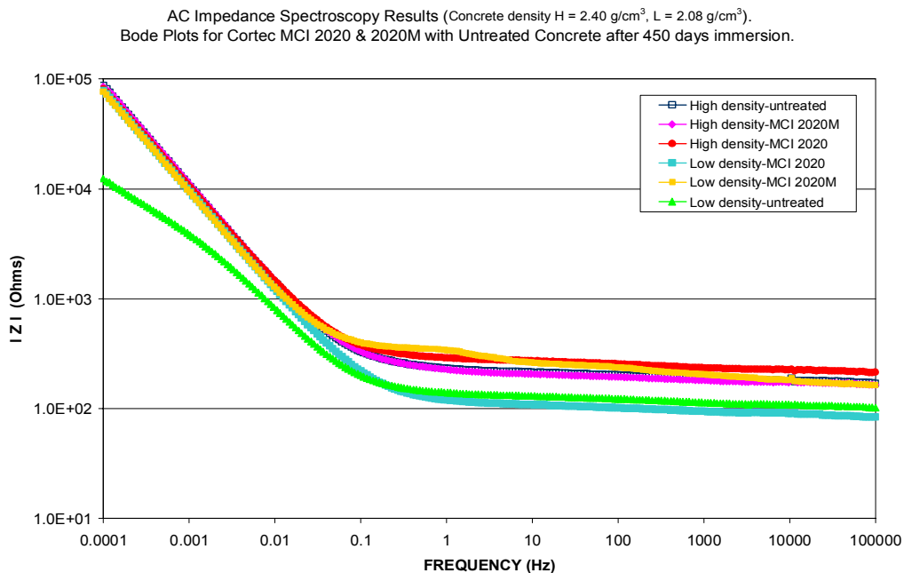
Figure 8 - EIS Bode plot for MCI 2020 treated & untreated concrete after 450 days of testing.
