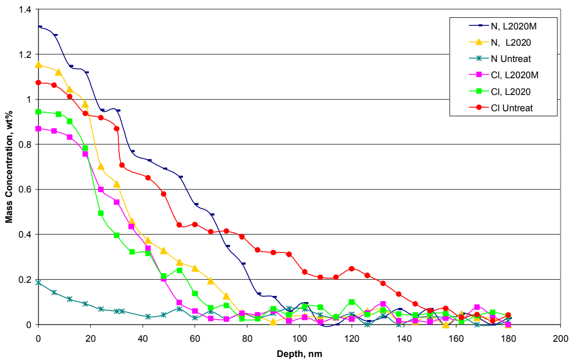
Figure 19 – XPS depth profiling showing mass concentration weight percentage of chloride and nitrogen for test samples.
