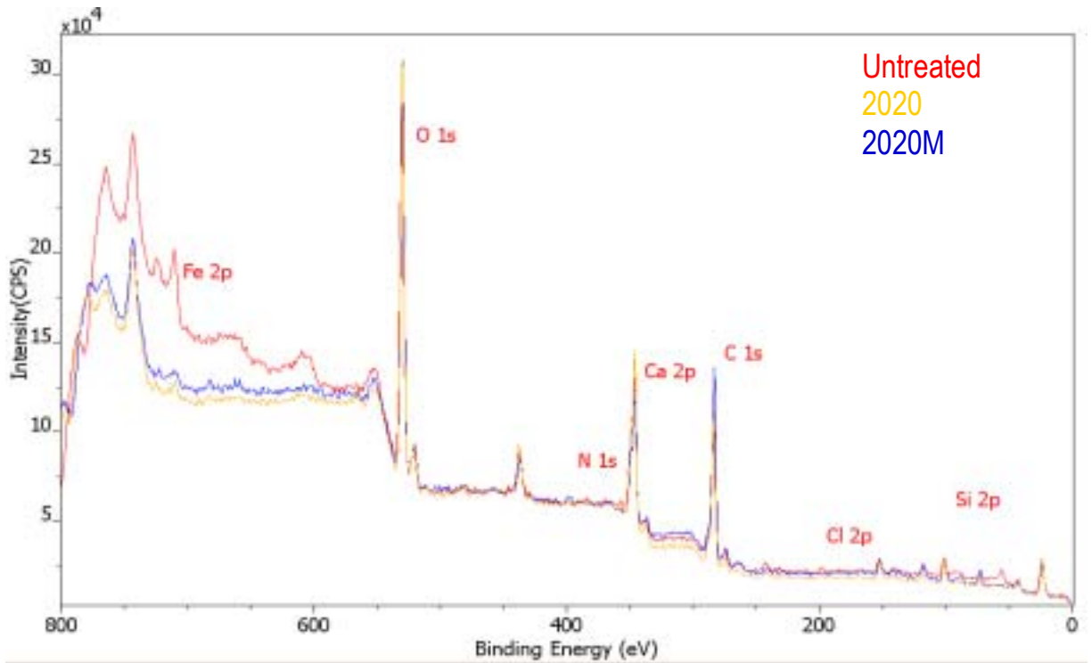
Figure 17 – XPS analysis on concrete samples after 500 days, 120 seconds etching.
