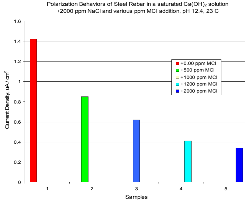
Figure 4 - Polarization behavior of steel rebar in a saturated Ca(OH) 2 solution with 2000 ppm NaCl and various ppm MCI 2020M additions, pH 12.4, 23 °C.
