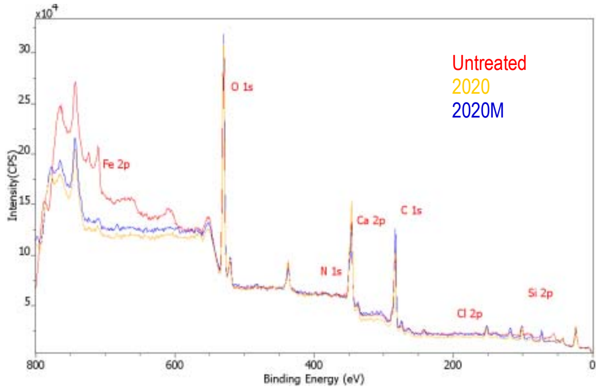
Figure 18 – XPS analysis on concrete samples after 500 days, 240 seconds etching.
