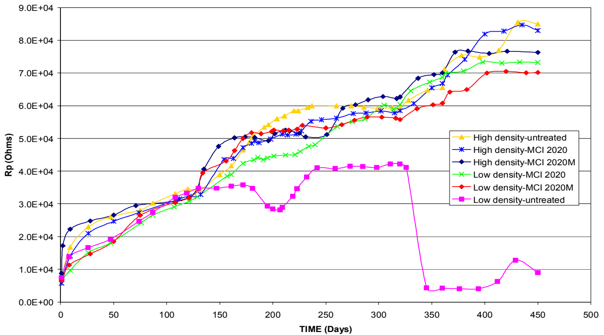
Figure 6 - Comparison of polarization resistance ( R_p ) for MCI treated & untreated concrete samples.
