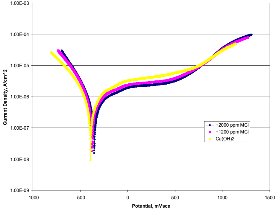
Figure 2 - Polarization behavior of steel rebar in a saturated \text{Ca(OH)}_2 solution with 2000 ppm NaCl and various ppm MCI 2020M additions, pH 12.4, 23 °C.
