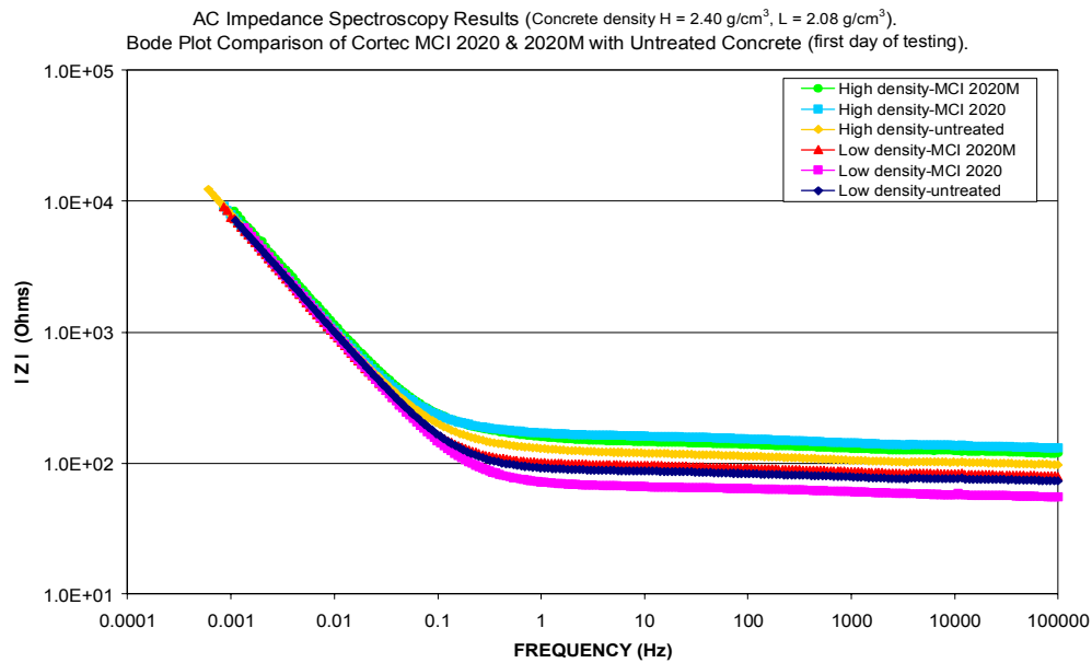
Figure 7 - EIS Bode plot for MCI 2020 treated & untreated concrete on day 1 of testing.
